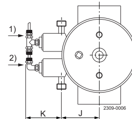
1) CIP valve
